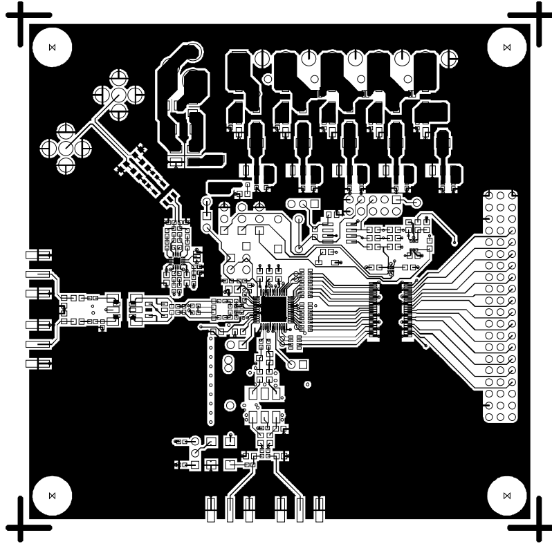
Figure 58. Evaluation Board Layout, Primary Side
