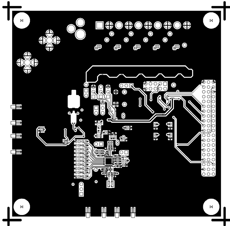
Figure 59. Evaluation Board Layout, Secondary Side (Mirrored Image)
