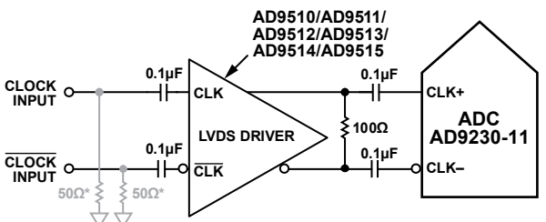
Figure 26. Differential LVDS Sample Clock
