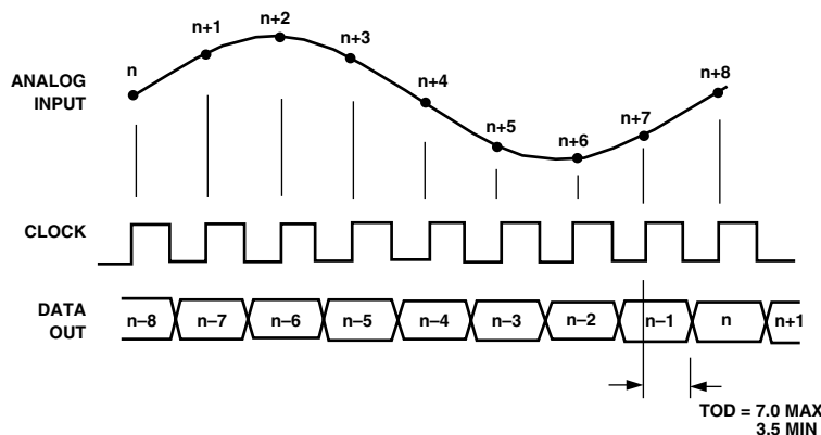
Figure 1. Timing Diagram
