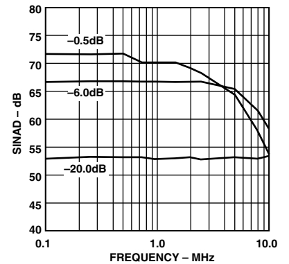
TPC 15. SINAD vs. Input Frequency (Input Span = 5.0 V p-p, V CM = 2.5 V)
