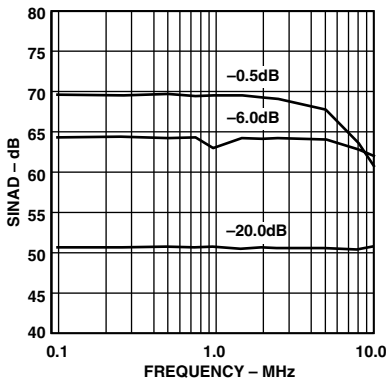
TPC 13. SINAD vs. Input Frequency (Input Span = 2.0 V p-p, V CM = 2.5 V)
