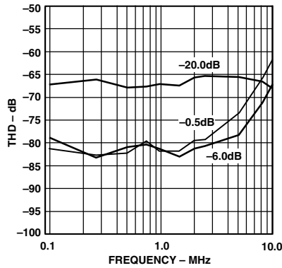
TPC 14. THD vs. Input Frequency (Input Span = 2.0 V p-p, V CM = 2.5 V)
