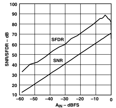
TPC 18. SNR/SFDR vs. A IN (Input Amplitude) (f IN = 1.5 MHz, Input Span = 2 V p-p, V CM = 2.5 V)
