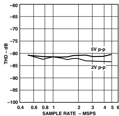
TPC 17. THD vs. Sample Rate (A IN = -0.5 dB, f IN = 500 kHz, V CM = 2.5 V)
