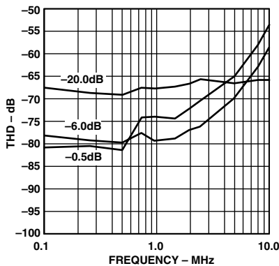
TPC 16. THD vs. Input Frequency (Input Span = 5.0 V p-p, V CM = 2.5 V)
