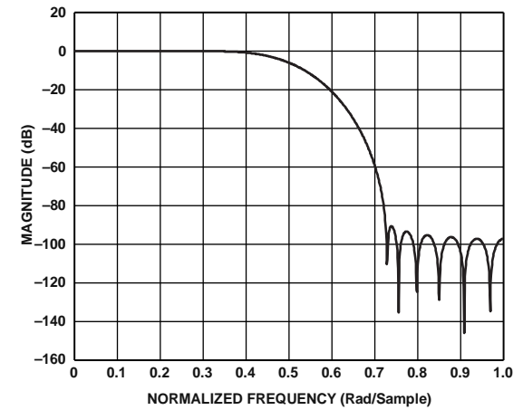
Figure 116. Second 2x Half-Band 45% Filter Response
