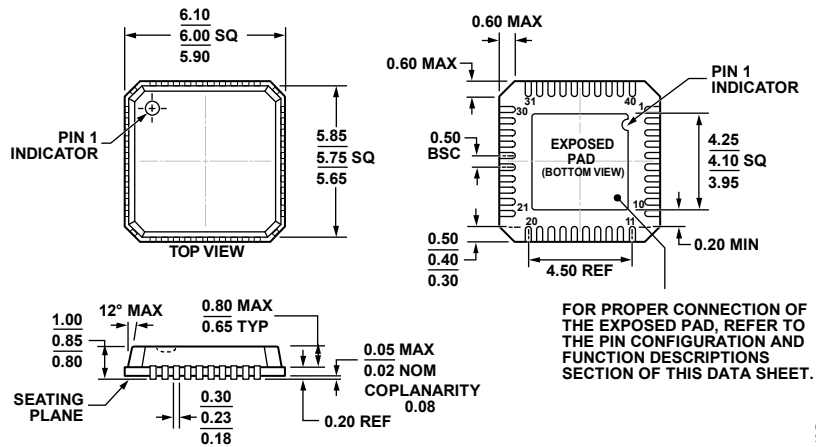
Figure 111. 40-Lead Lead Frame Chip Scale Package [LFCSP] 6 mm x 6 mm and 0.85 mm Package Height (CP-40-1) Dimensions shown in millimeters
