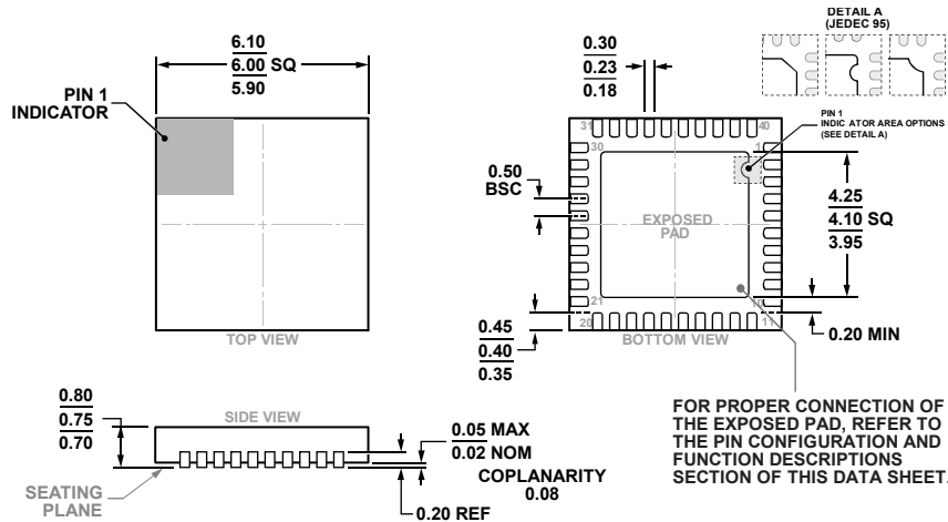
Figure 112. 40-Lead Lead Frame Chip Scale Package [LFCSP] 6 mm x 6 mm and 0.75 mm Package Height (CP-40-9) Dimensions shown in millimeters
