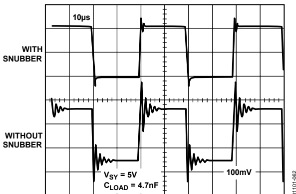
Figure 62. Overshoot and Ringing are Substantially Reduced Using a Snubber Network
