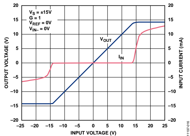
Figure 16. Input Overvoltage Performance; G = 1 , V_S = \pm 15V
