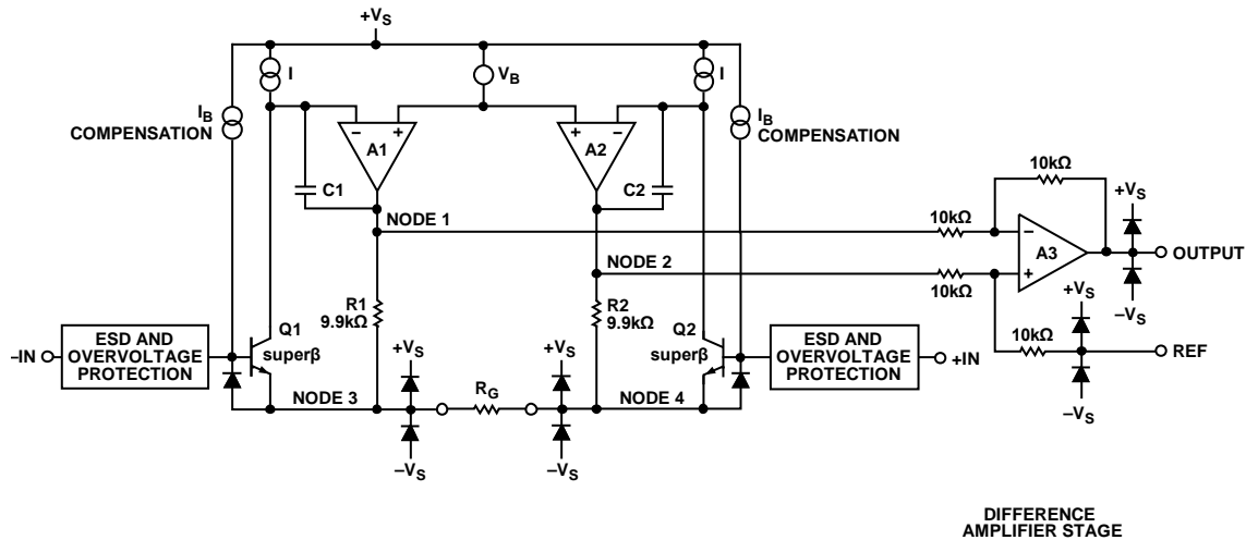
Figure 56. Simplified Schematic
