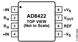
Figure 3. 8-Lead MSOP and 8-Lead SOIC_N Pin Configuration
