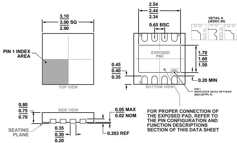
Figure 68. 8-Lead Lead Frame Chip Scale Package [LFCSP] 3 mm x 3 mm Body and 0.75 mm Package Height (CP-8-19)
