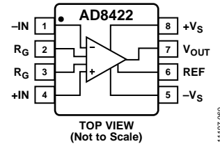
Figure 58. Pinout Diagram
