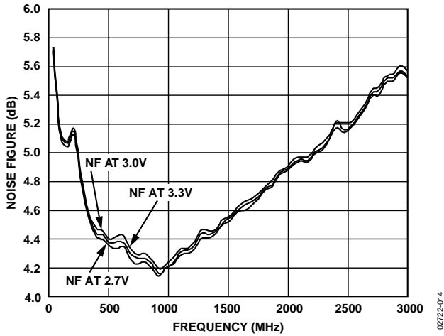
Figure 15. Noise Figure vs. Frequency, V_S = 2.7V, 3V, \text{ and } 3.3V, T_A = 25^\circ C
