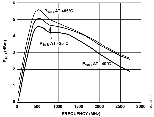
Figure 12. P_{1dB} vs. Frequency, V_S = 3V, T_A = -40^\circ C, +25^\circ C, and +85^\circ C
