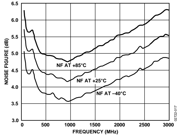
Figure 18. Noise Figure vs. Frequency, V_S = 3V, T_A = -40^\circ C, +25^\circ C, \text{ and } +85^\circ C
