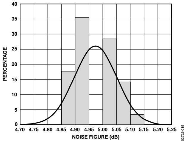
Figure 16. Distribution of Noise Figure, V_S = 3V, T_A = 25^\circ C, f = 2.2 GHz
