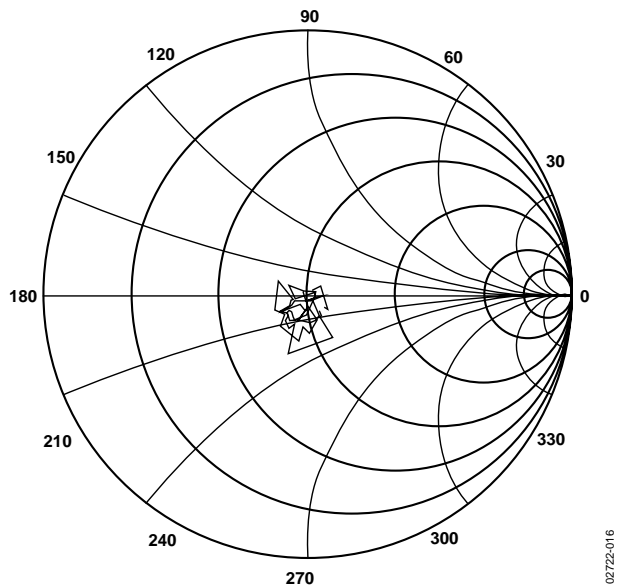
Figure 17. S_{11} vs. Frequency, V_S = 5V, T_A = 25^\circ C, 100 MHz \leq f \leq 3 GHz
