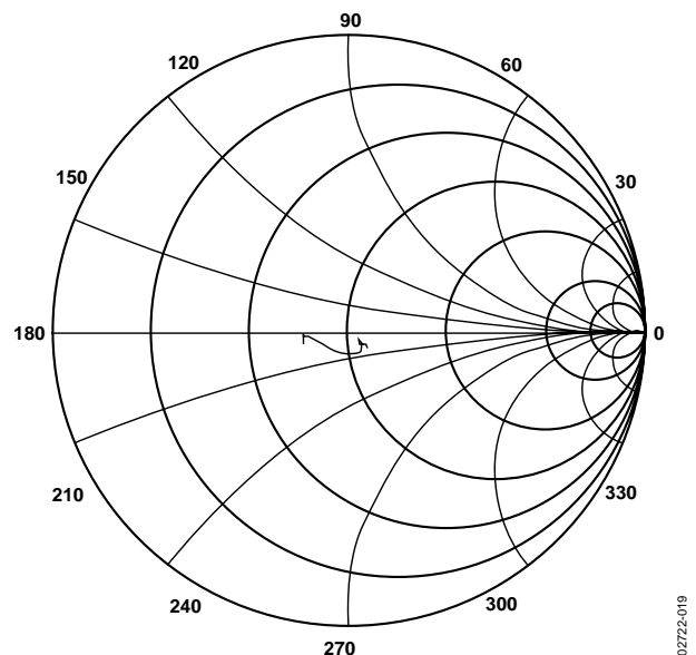
Figure 20. S_{22} vs. Frequency, V_S = 5V, T_A = 25^\circ C, 100 MHz \leq f \leq 3 GHz
