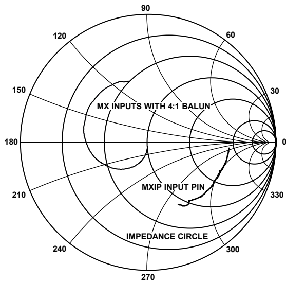
Figure 44. S_{11} of Mixer Input vs. F_{IF} , F_F = 50 \text{ MHz} to 1 \text{ GHz} , V_{GIN} = 0.7 V , V_{POS} = 5 V (With and Without Balun)
