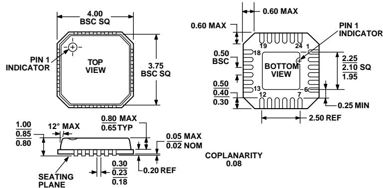
Figure 42. 24-Lead Lead Frame Chip Scale Package [LFCS] (CP-24)
