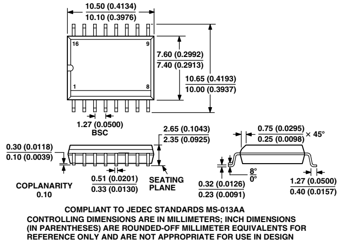
16-Lead Standard Small Outline Package [SOIC] Wide Body (R-16)
