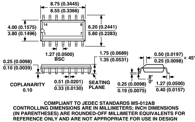
14-Lead Standard Small Outline Package [SOIC] Narrow Body (R-14)
