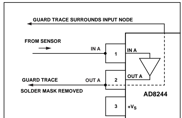
Figure 40. Guarding with the AD8244
