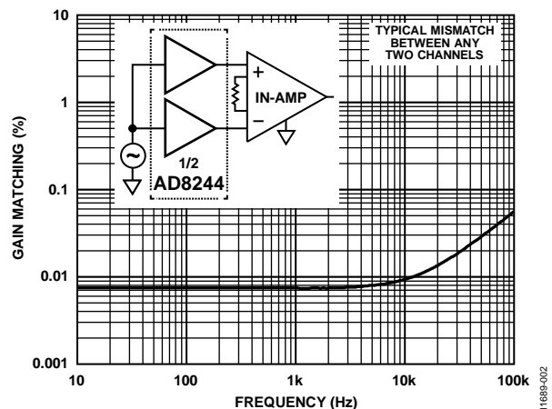
Figure 2. Gain Matching vs. Frequency
