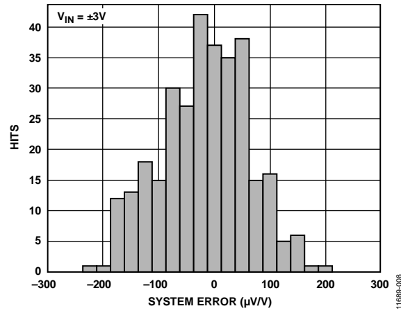
Figure 8. Typical Distribution of System Error
