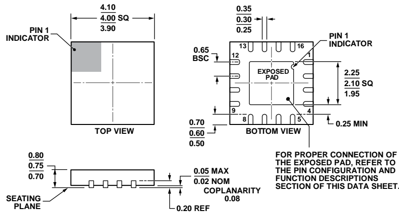
Figure 57. 16-Lead Lead Frame Chip Scale Package [LFCSP_WQ] 4 mm × 4 mm Body, Very Very Thin Quad (CP-16-23) Dimensions shown in millimeters
