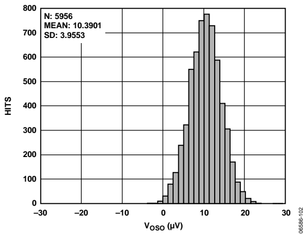
Figure 5. Instrumentation Amplifier Output Offset Voltage Distribution
