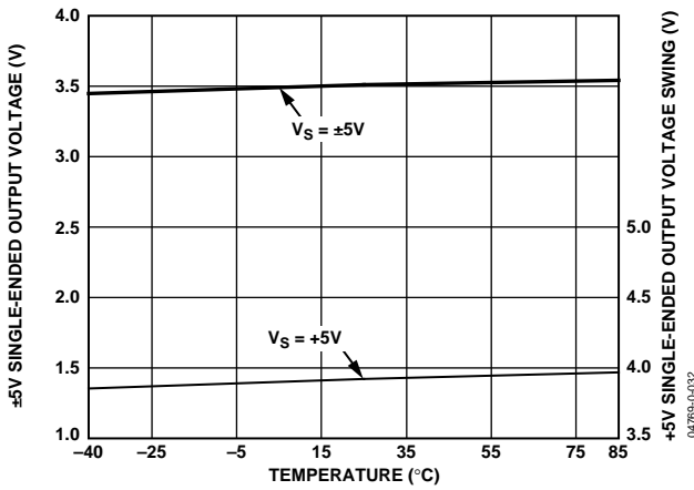
Figure 30. Positive Output Saturation Voltage vs. Temperature
