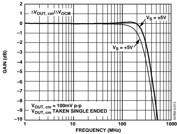
Figure 25. V_{OCM} Frequency Response for Various Power Supply Voltages
