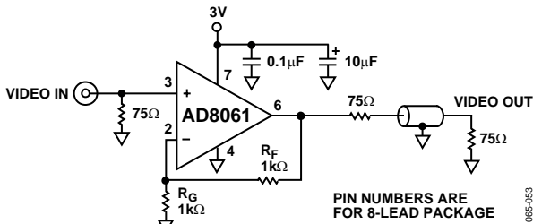
Figure 53. Single 3 V Sync Stripper Using AD8061
