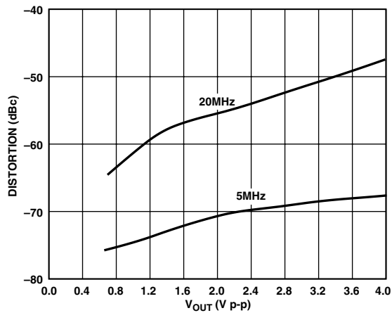
TPC 21. Distortion vs. V_{OUT} @ 20 MHz, 5 MHz, R_L = 150\ \Omega , V_S = \pm 5.0\text{ V}
