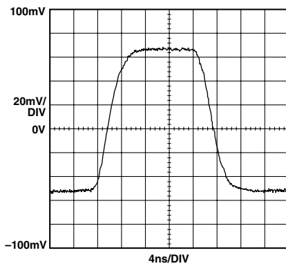
TPC 14. Small Signal Step Response G = -1 , R_L = 1\text{ k}\Omega
