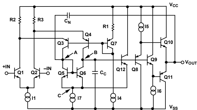
Figure 31. AD797 Simplified Schematic
