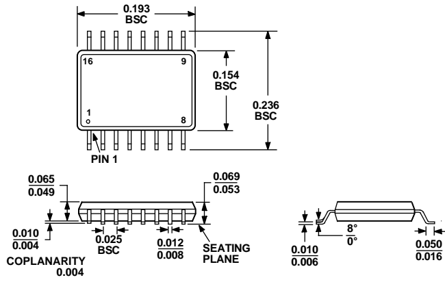
Figure 40. 16-Lead Shrink Small Outline Package [QSOP] (RQ-16) Dimensions shown in inches
