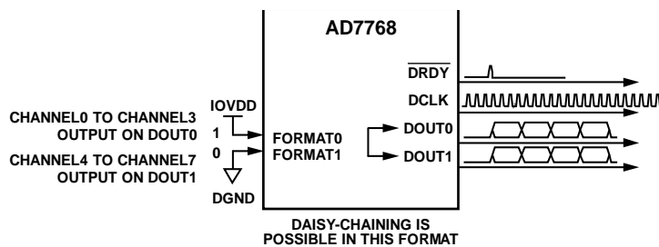
Figure 93. AD7768 FORMATx = 01, Two Data Output Pins
