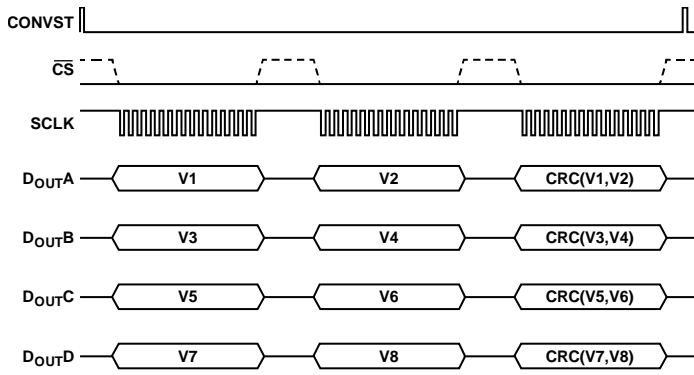
Figure 115. Serial Interface ADC Reading with CRC On, Four D OUTX Lines
