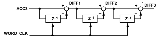
Figure 26. Differentiator
