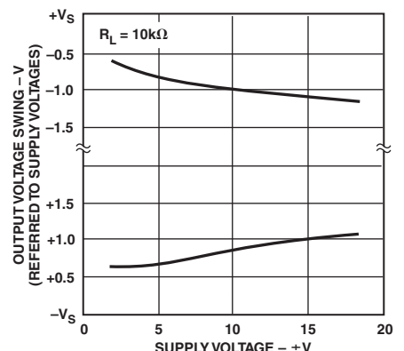
TPC 18. Output Voltage Swing vs. Supply Voltage
