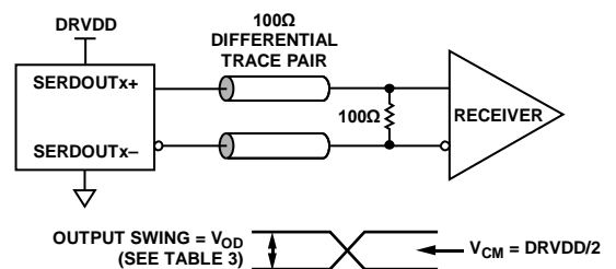
Figure 53. DC-Coupled Digital Output Termination Example
