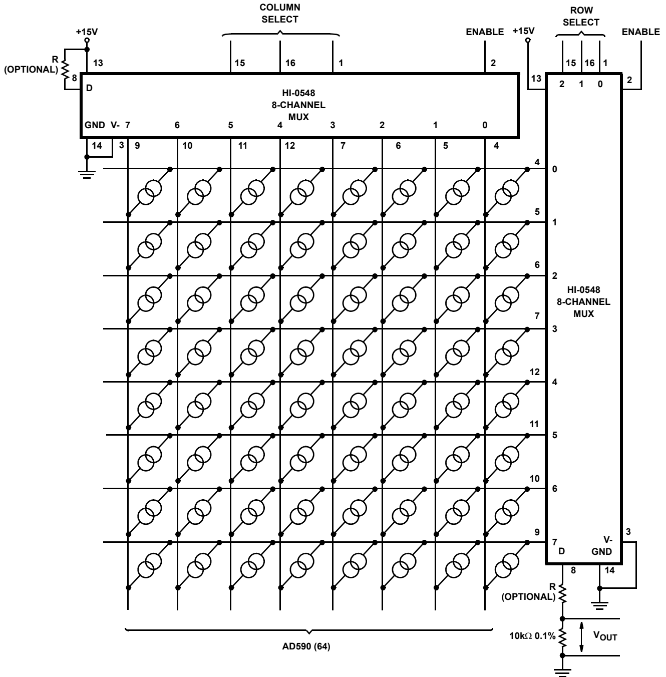
FIGURE 17. MULTIPLEXING SENSORS
