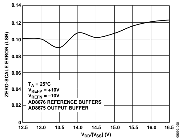
Figure 19. Zero-Scale Error vs. Supply Voltage, ±10 V Span
