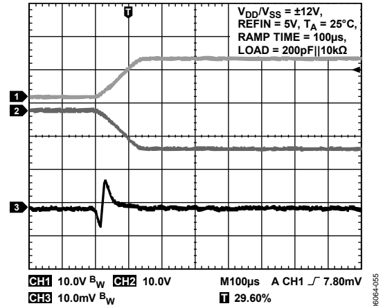
Figure 30. V_{OUTx} vs. V_{DD}/V_{SS} on Power-Up
