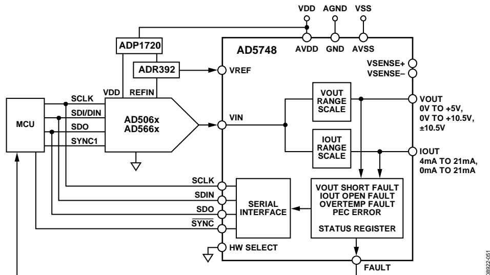
Figure 49. Typical System Configuration in Software Mode (Pull-Up Resistors Not Shown for Open-Drain Outputs)
