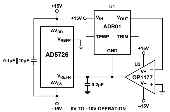
Figure 25. Unipolar -10 V Operation
