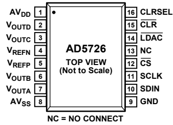
Figure 5. Pin Configuration
