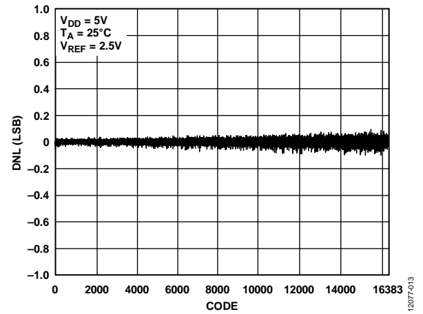
Figure 13. AD5692R DNL
