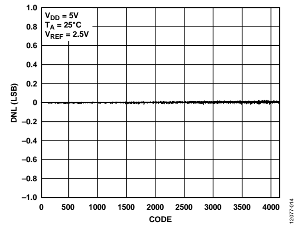
Figure 14. AD5691R DNL
