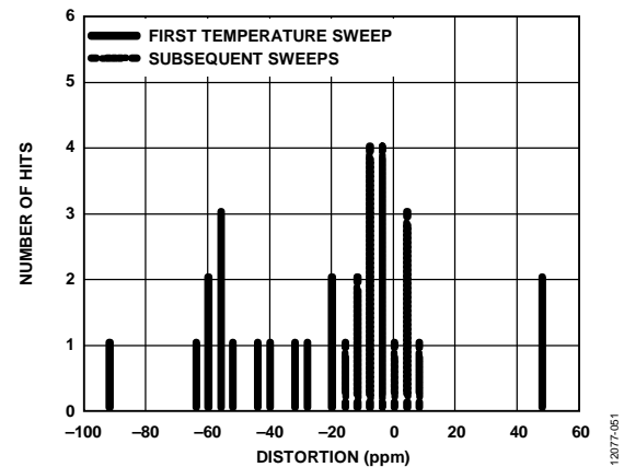
Figure 50. Thermal Hysteresis
