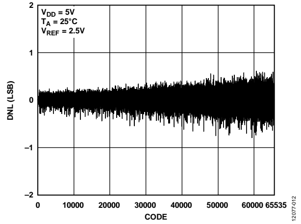
Figure 12. AD5693R/AD5693 DNL
