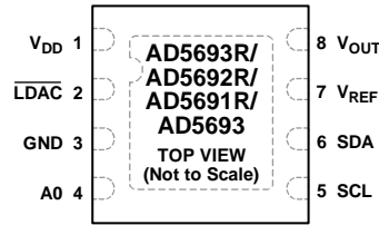
Figure 6. AD5693R/AD5692R/AD5691R/AD5693 Pin Configuration, 8-Lead LFCSP, LDAC Option
