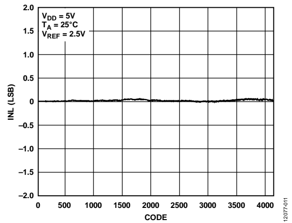
Figure 11. AD5691R INL
