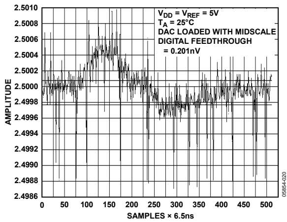
Figure 18. Digital Feedthrough
