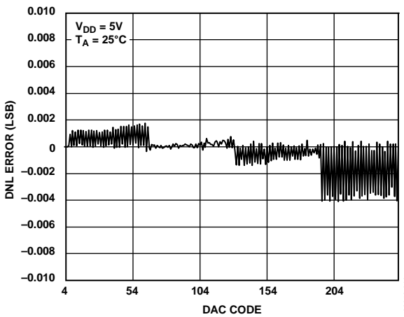
Figure 13. Typical AD5601 DNL
