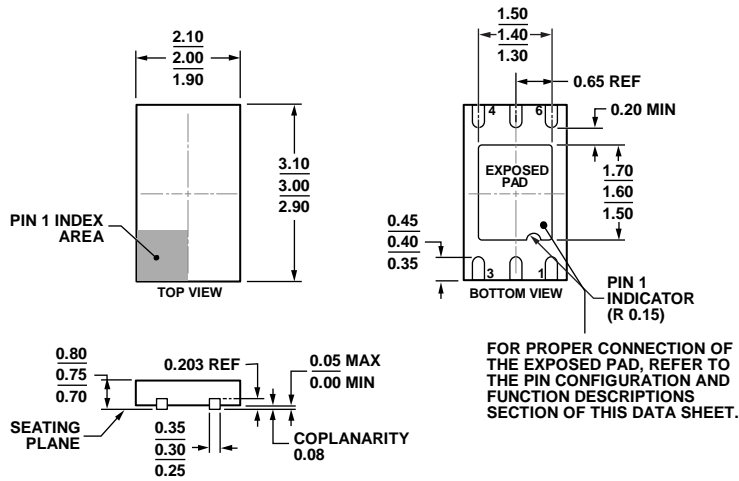
Figure 55. 6-Lead Lead Frame Chip Scale Package [LF CSP_WD] 2.00 x 3.00 mm Body, Very Very Thin, Dual Lead (CP-6-5) Dimensions shown in millimeters
