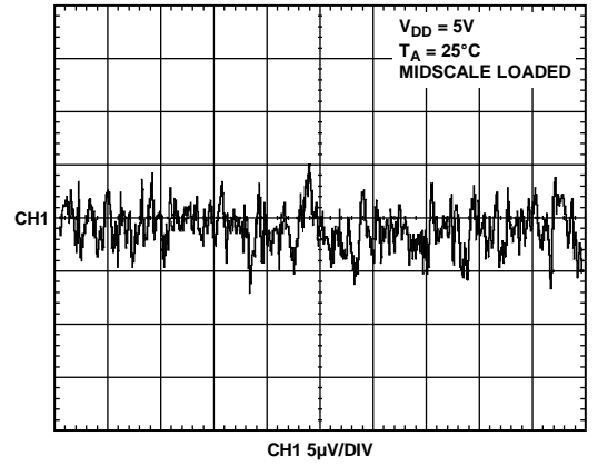
Figure 20. 1/f Noise, 0.1 Hz to 10 Hz Bandwidth
