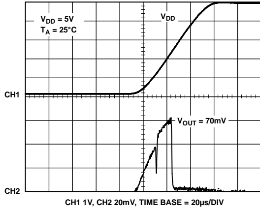
Figure 17. Power-On Reset to 0V
