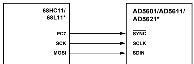
Figure 47. AD5601/AD5611/AD5621 to 68HC11/68L11 Interface
