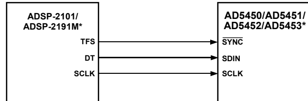
Figure 57. ADSP-2101/ADSP-2191M-to-AD5450/AD5451/AD5452/AD5453 Interface
