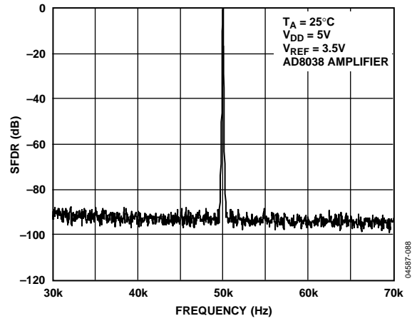
Figure 39. Narrow-Band SFDR, f_{OUT} = 50\text{ kHz} , Clock = 1 MHz
