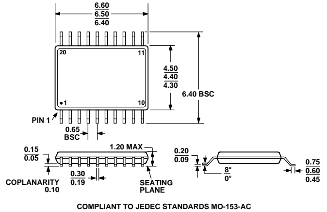
COMPLIANT TO JEDEC STANDARDS MO-153-AC Figure 64. 20-Lead Thin Shrink Small Outline Package [TSSOP] (RU-20) Dimensions shown in millimeters
