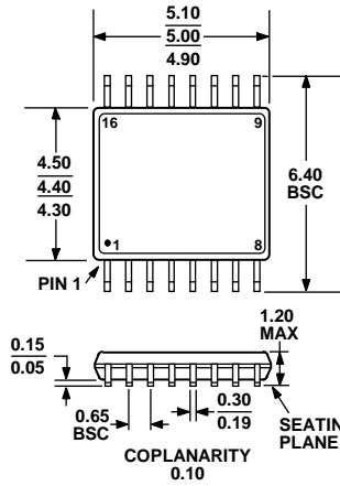
COMPLIANT TO JEDEC STANDARDS MO-153-AB Figure 63. 16-Lead Thin Shrink Small Outline Package [TSSOP] (RU-16) Dimensions shown in millimeters
