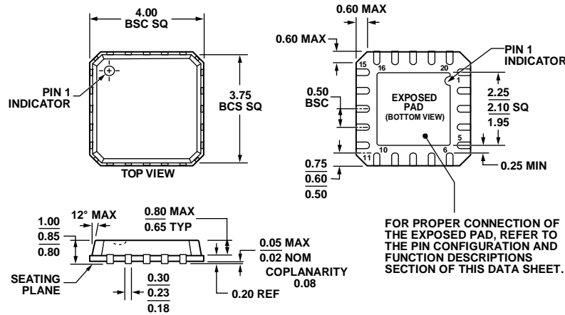
COMPLIANT TO JEDEC STANDARDS MO-220-VGGD-1 Figure 65. 20-Lead Lead Frame Chip Scale Package [LFCS_P_VQ] 4 mm x 4 mm Body, Very Thin Quad (CP-20-1) Dimensions shown in millimeters
