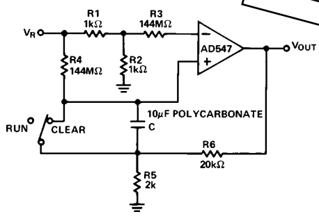
Figure 38. Long Interval Timer-1,000 Seconds
