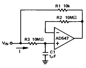
Figure 37. Capacitance Multiplier
