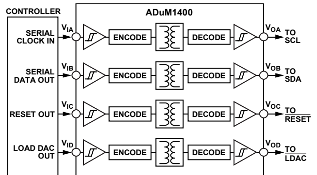
Figure 51. Isolated Interface
