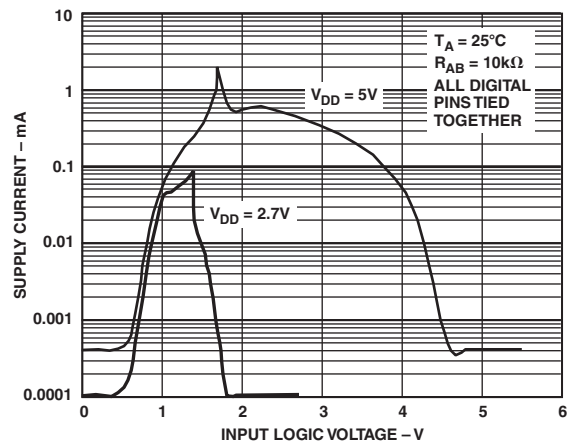
TPC 12. Supply Current vs. Digital Input Voltage
