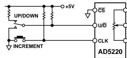
Figure 1. Typical Push-Button Control Application
