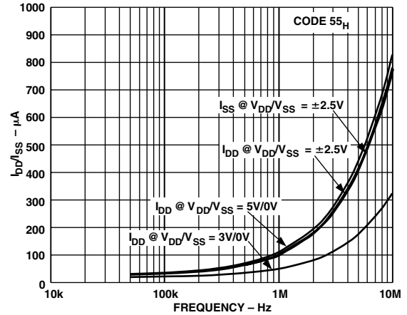
TPC 10. 10 k \Omega Supply Current vs. Clock Frequency
