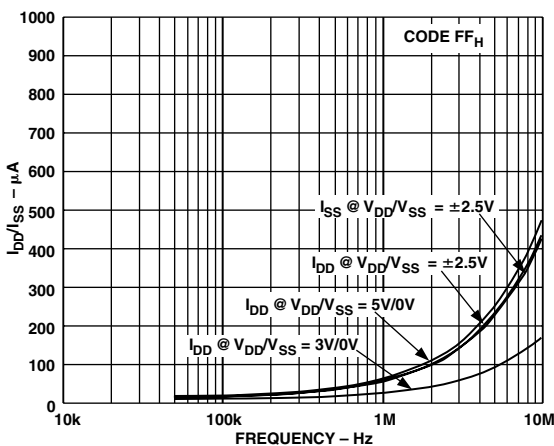
TPC 9. 10 k \Omega Supply Current vs. Clock Frequency
