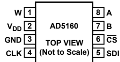
Figure 3. Pin Configuration
