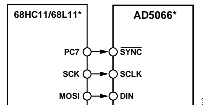
Figure 44. AD5066 to 68HC11/68L11 Interface
