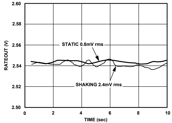
Figure 26. Random Vibration (Lateral) 10 kHz to 20 kHz at 0.01 g/\sqrt{Hz} with 60 Hz Sampling and 0.5 sec Averaging
