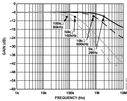
Figure 26. -3\text{ dB} Bandwidth @ Code = 0 \times 80
