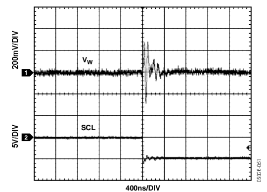
Figure 29. Digital Feedthrough
