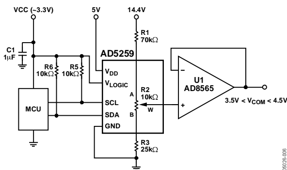
Figure 46. V_{COM} Adjustment Application
