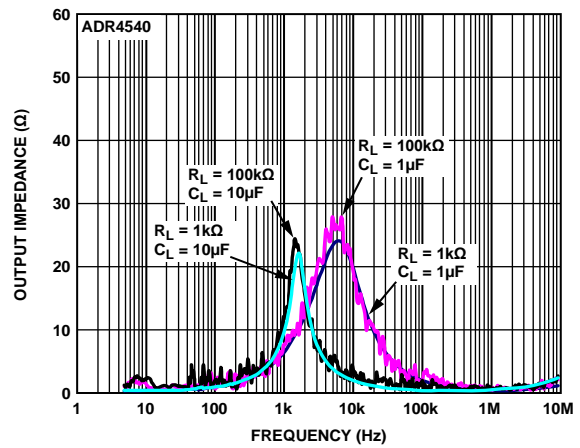
Figure 79. ADR4540 Output Impedance vs. Frequency
