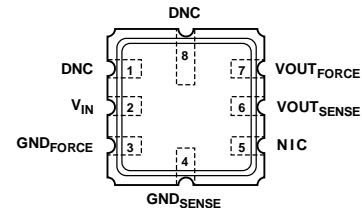
Figure 2. 8-Lead LCC Pin Configuration
