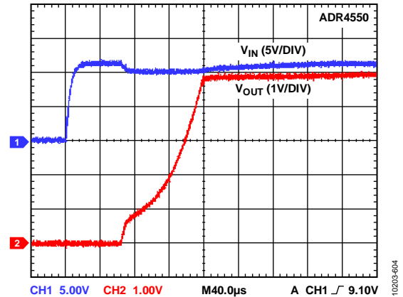
Figure 89. ADR4550 Output Voltage Start-Up Response
