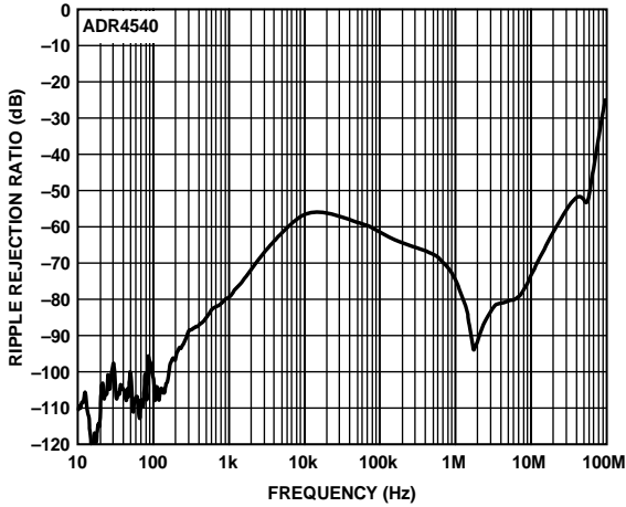
Figure 76. ADR4540 Ripple Rejection Ratio vs. Frequency
