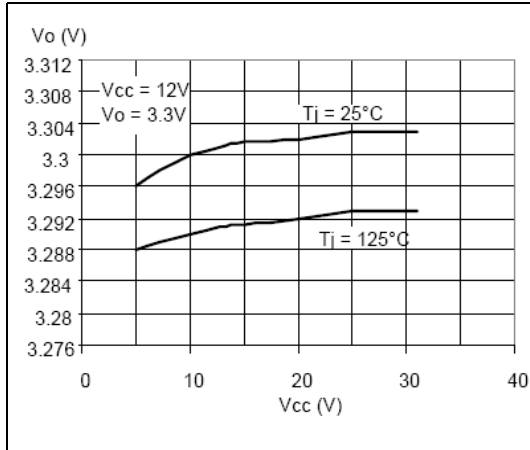
Figure 2. Line regulator
