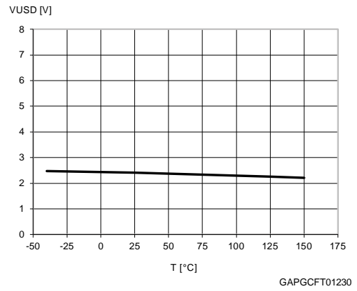
Figure 24: Undervoltage shutdown
