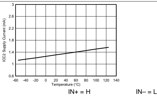
Figure 9. I_{CC2} Supply Current vs Temperature
