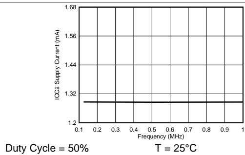
Figure 10. I_{CC2} Supply Current vs Input Frequency
