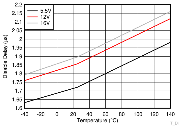
Figure 6-13. Disable Delay
