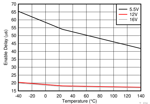
Figure 6-12. Enable Delay
