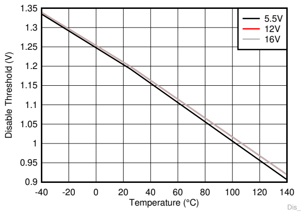
Figure 6-11. Disable Threshold
