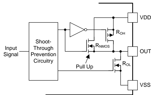
Figure 31. Output Stage
